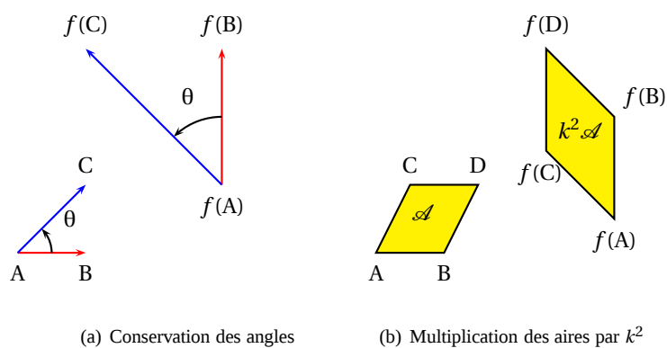
FIGURE 28.7 – Similitudes directes
