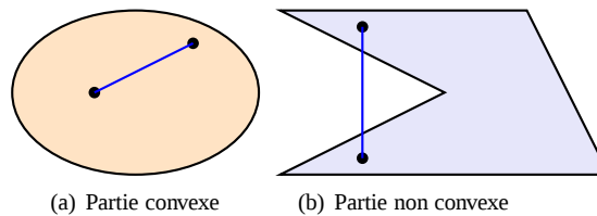
FIGURE 28.3 – Parties convexes
