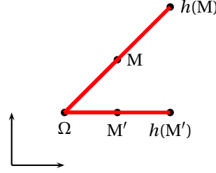
FIGURE 28.5 – Homothétie affine
