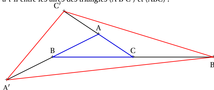
FIGURE 2.18 – Exercice 2.27
